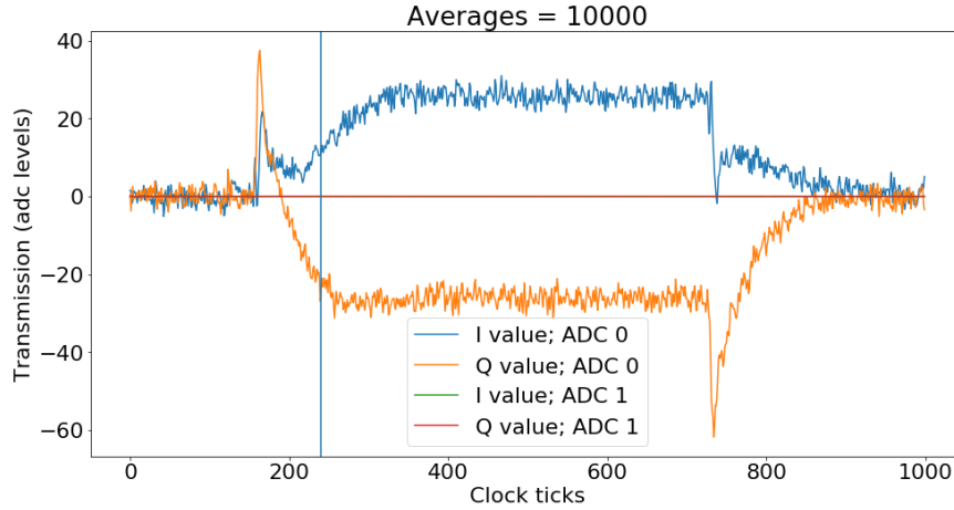
Figure 2: Loopback measurement used to optimize the readout timing.
